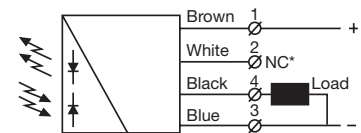
*Do not connect white wire SMP / SMPF / SMRR 7600 (load as PNP)
