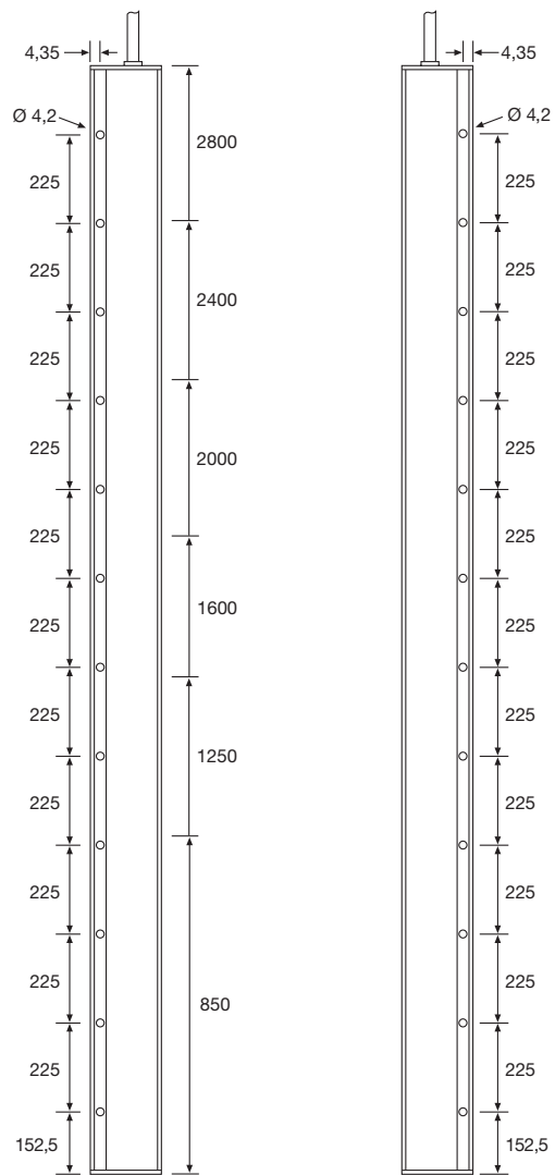
SGR Rear View
